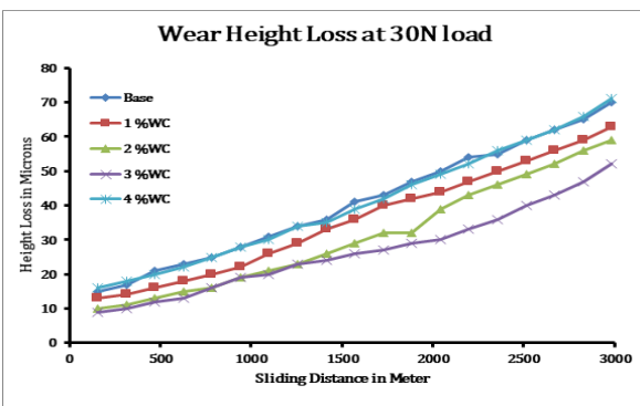
Figure 4: Wear at 30 N
