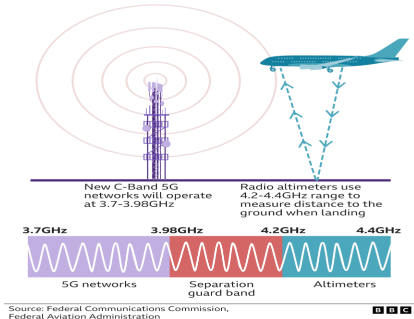
Figure 2: Separation guard band between 5 network and altimeters
