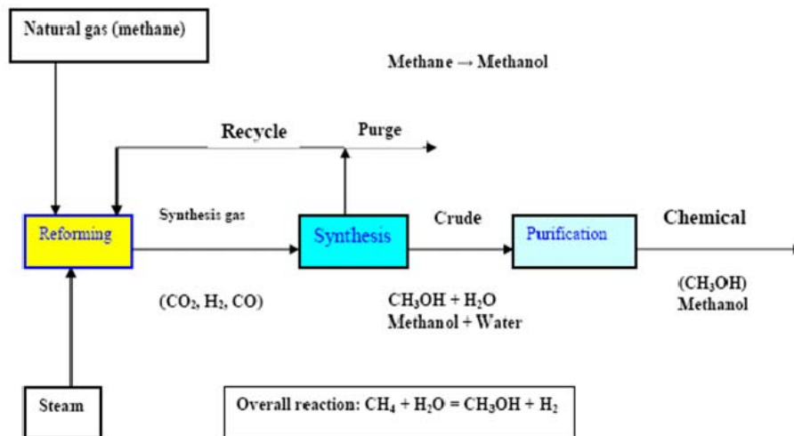
Figure 2. Schematic diagram shows methanol production (Omer, 2006).
