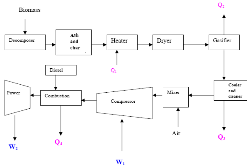
Figure 7. Advanced biomass power with diesel engine (Omer, 2006).
