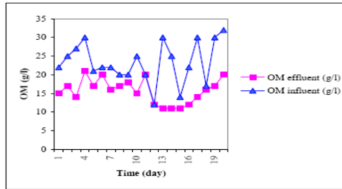
Figure 5. Organic matters before and after treatment in digester (Omer, 2006).
