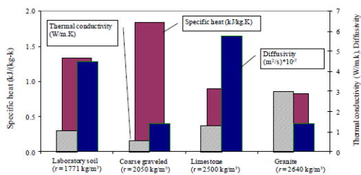
Figure 1. Measured thermal properties for different soils
