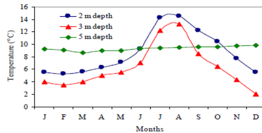
Figure 7. Ground temperatures throughout the year
