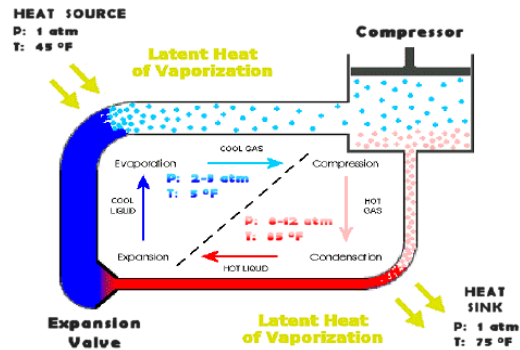
Figure 6. Heat pump works by promoting the evaporation and condensation of a refrigerant
