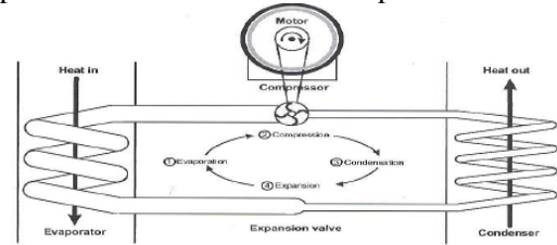
Figure 4. Ground source heat pumps
