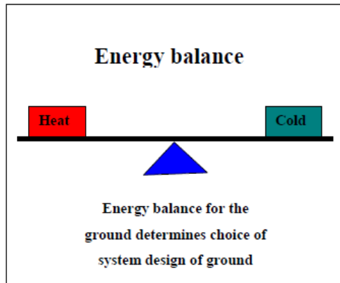
Figure 5. Energy balance for ground
