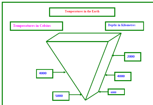
Fig. 3. Earth energy budget
